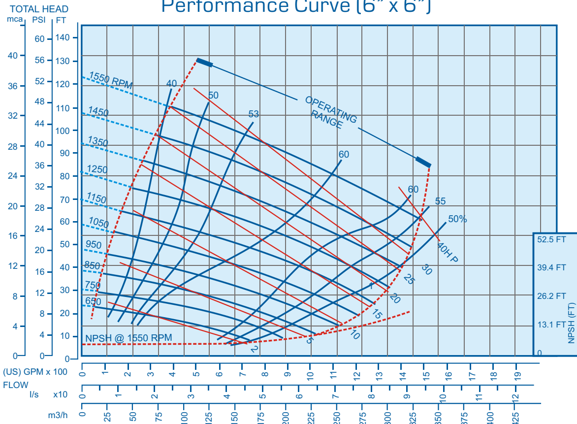
Performance Curve (6" x 6")
